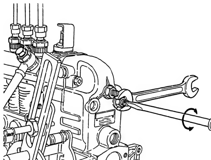
Fig. 86 Setting of damper spring
